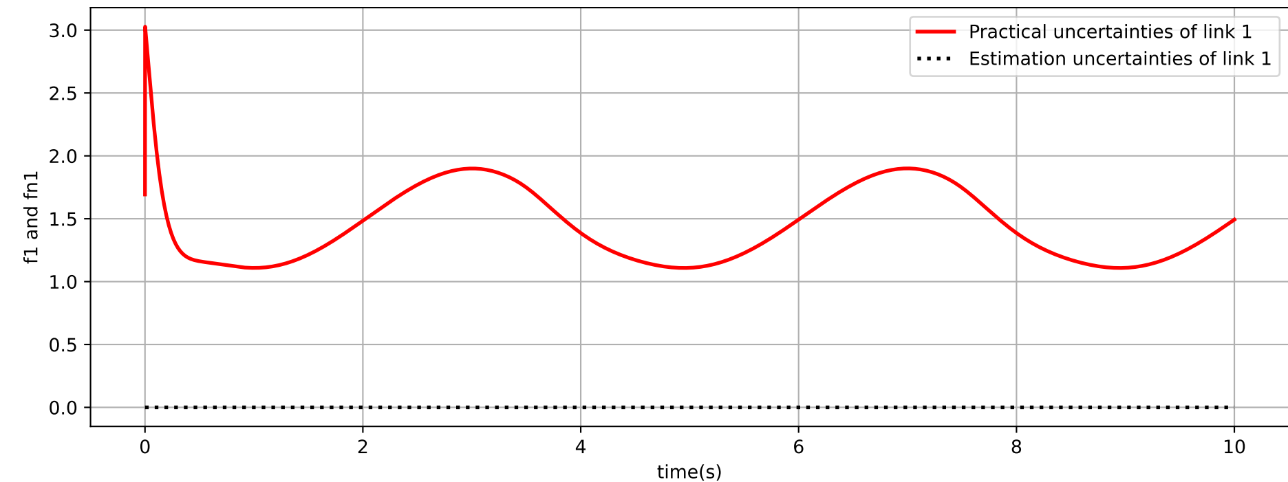
Disturbance Estimation Performance ( S=1 , S1=1 , m=5 )
